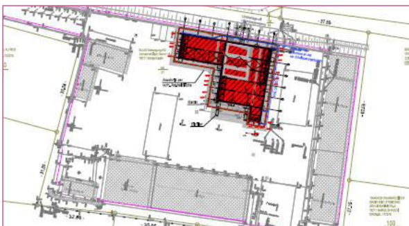
Lageplan der Konditionierungshalle in der Planungsphase Site map of the conditioning hall during the planning phase
